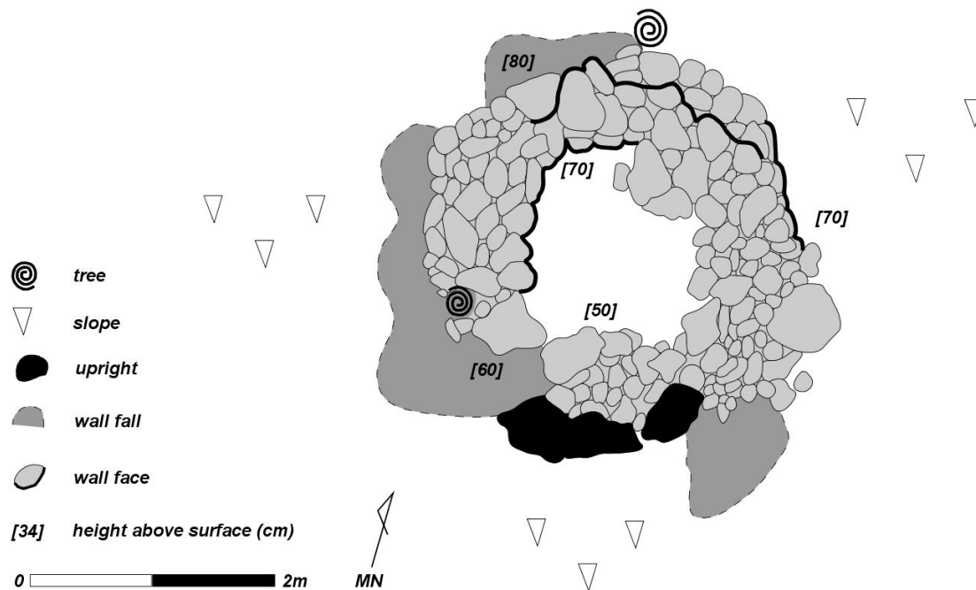
Figure 33. Current plan view drawing of Feature I.
