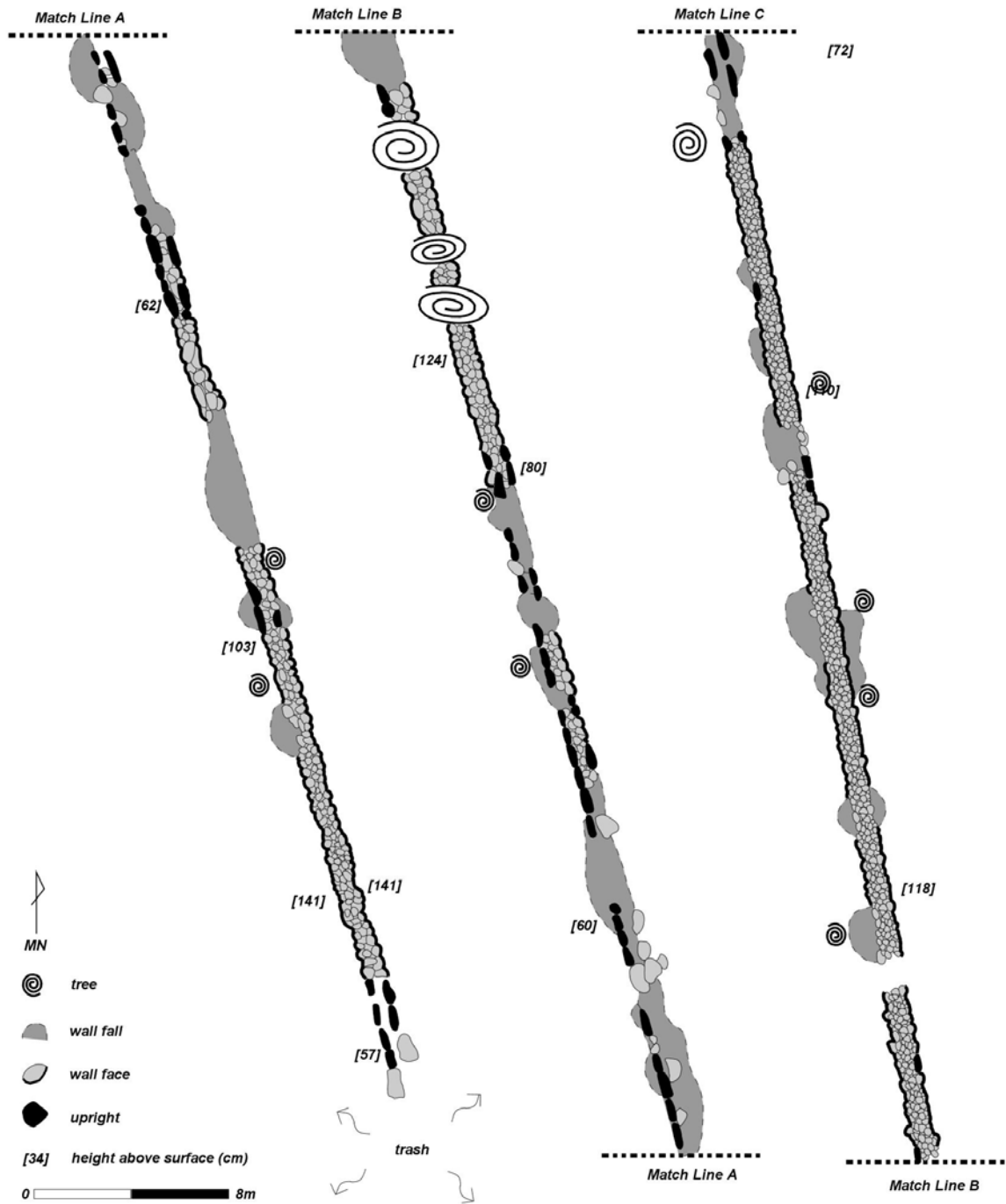
Figure 25. Current plan view drawing of Feature C, southern half of the wall. Note that upright slabs at the base of the wall are not visible in plan view where the wall is intact.
